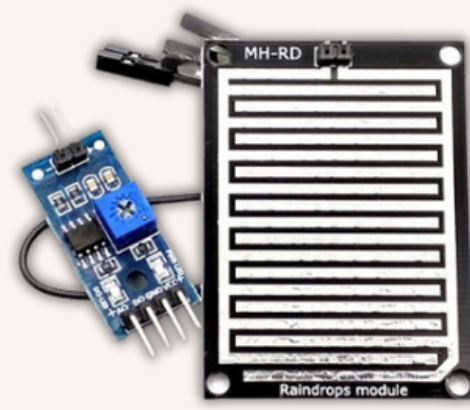
MH-RD Raindrop 49฿
